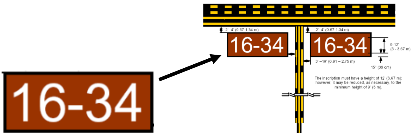
Surface Painting Holding Position Marking
