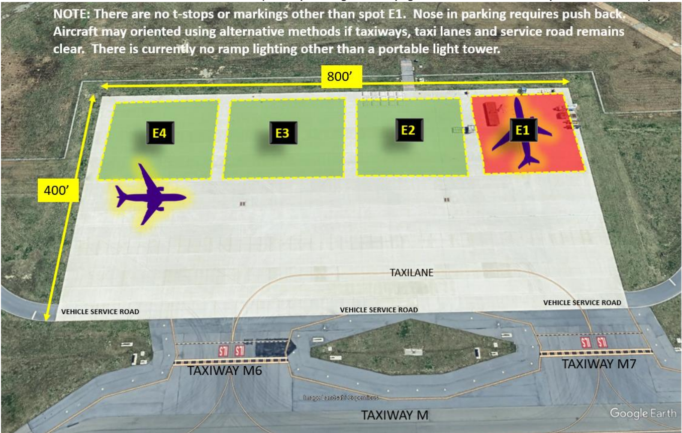
FIGURE 3a – EAST RAMP #1 (see Airport Diagram next page for location – contact Airport OPS for escort)
